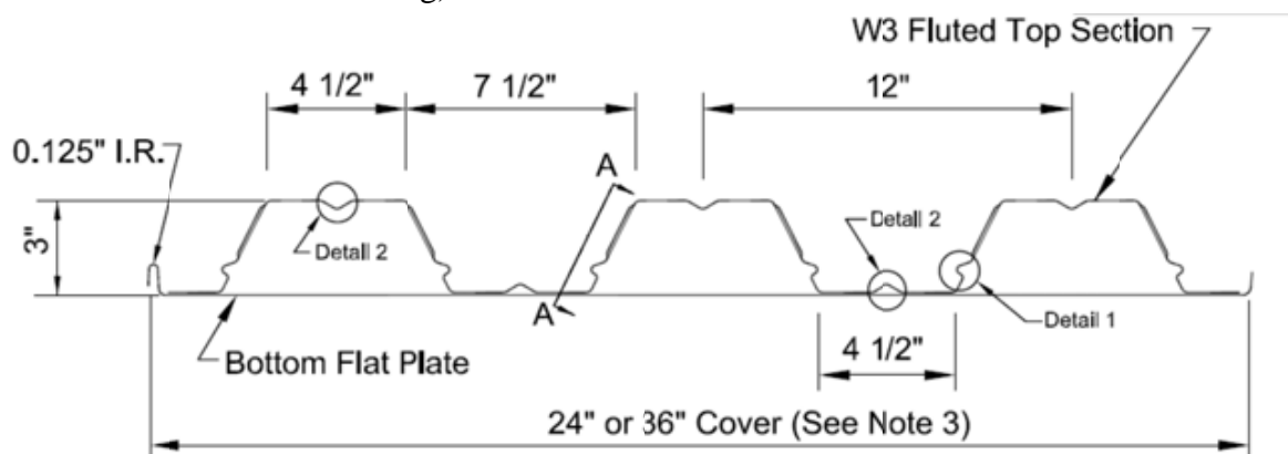
Figure 1 - Metal deck section drawing (supplied by client).
