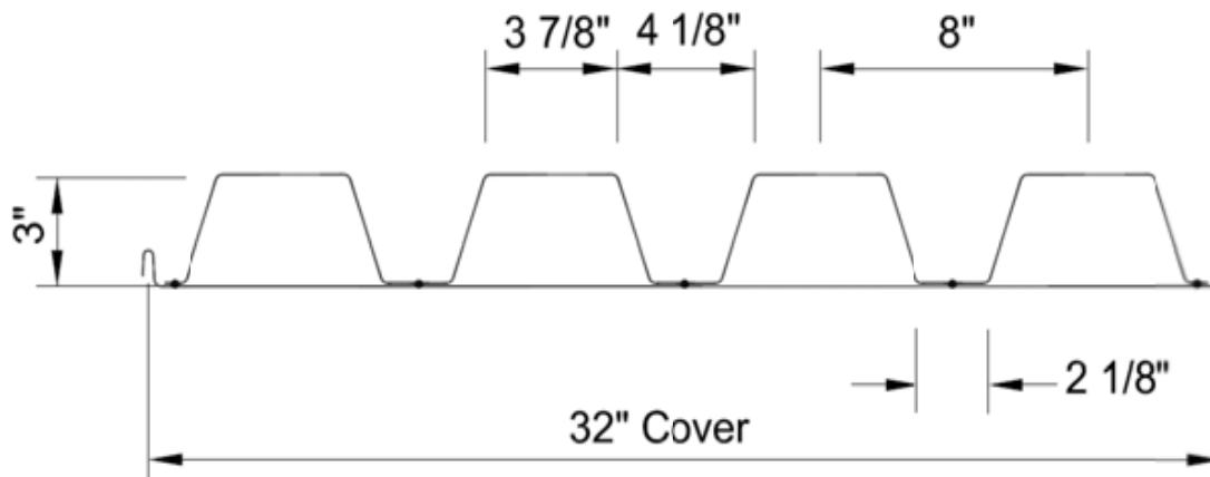
Figure 1 - Deck section detail (supplied by client).
