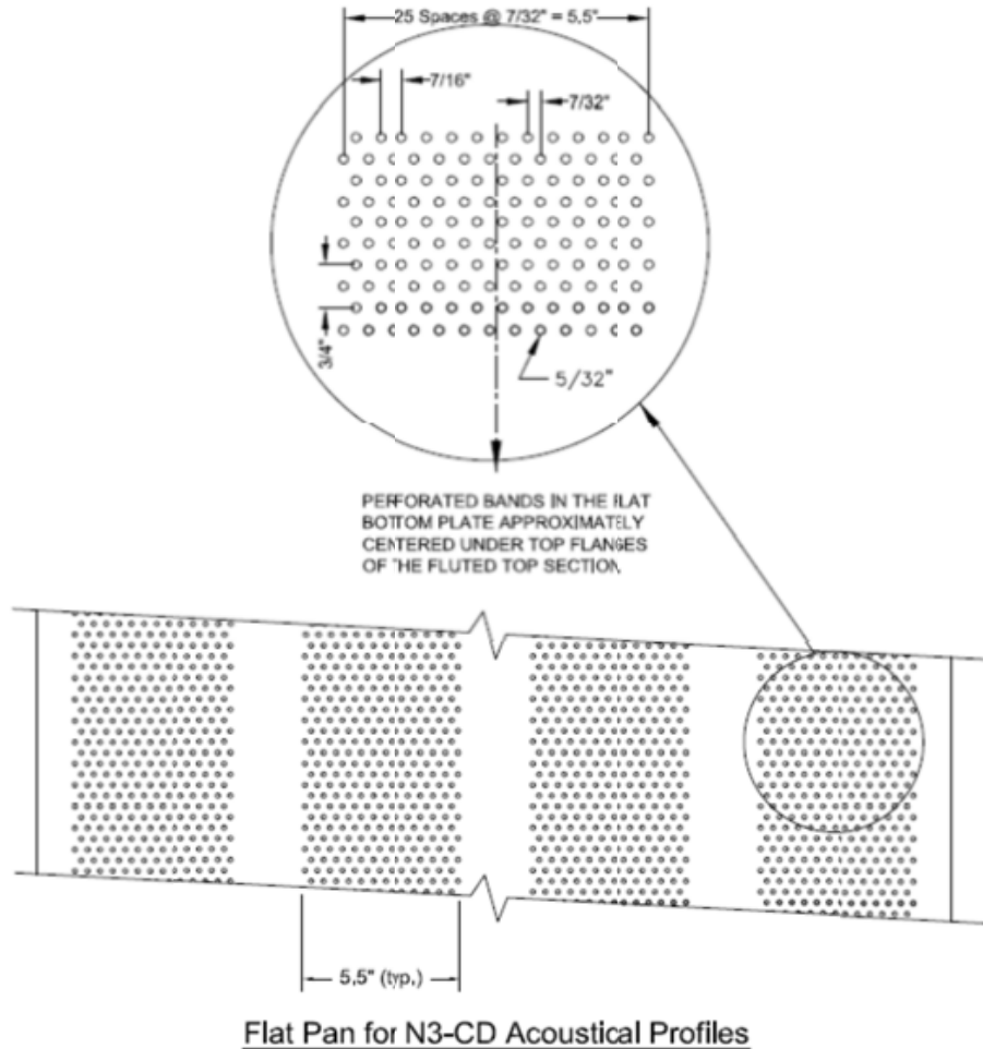
Figure 2 - Acoustical perforation detail (supplied by client).
