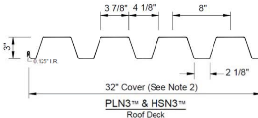
Figure 1 – Metal deck section drawing (supplied by client).
